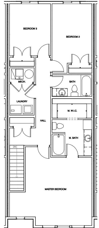
Upper Level
